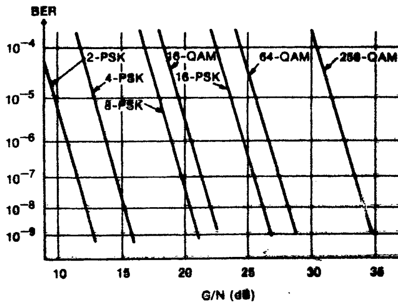
Figure 3.16 Error rates for PSK and QAM systems. (Reproduced with permission from IEEE © 1986. Noguchi, T., Y. Daido, and J. A. Nossek, Modulation Techniques for Microwave Digital Radio, IEEE Communications Magazine, vol. 24, no. 11, September 1986, pp. 21-30.)
